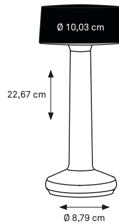
CYLINDER
