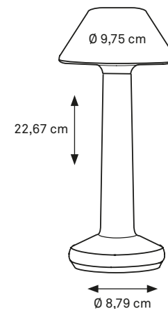
CAP OPAL
